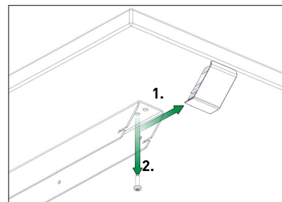
3 bureaublad losmaken
